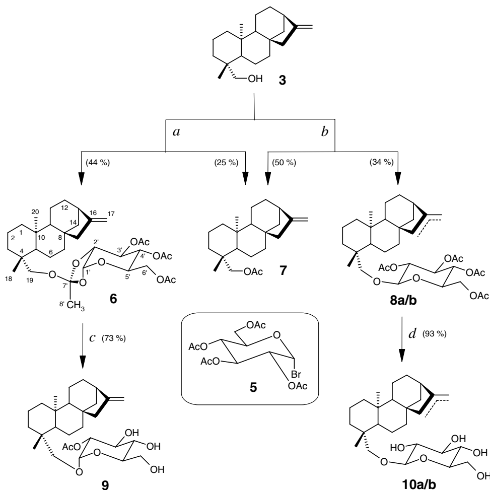
Scheme 2. Synthesis of the kaurane derivatives 6–10a/b from the alcohol 3 . (a) \text{C}_6\text{H}_5\text{Me} , ( 5 ), \text{Hg}(\text{CN})_2 , rt (24 h), 80^\circ\text{C} , 66 h; (b) \text{C}_6\text{H}_5\text{Me} , ( 5 ), \text{Hg}(\text{CN})_2 , 80^\circ\text{C} , 140 h; (c) \text{MeOH}/\text{H}_2\text{O}/\text{Et}_3\text{N} (8:1:1), rt, 24 h; (d) \text{MeO}^-\text{Na}^+ , \text{MeOH} , rt, 4 h.
